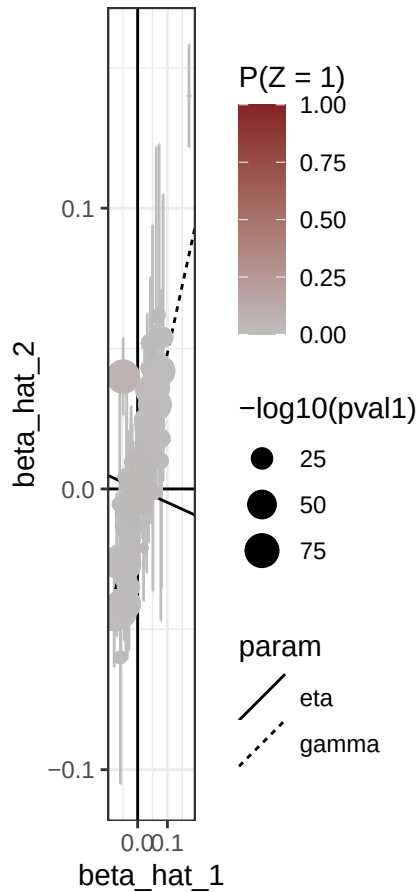
Causal Model
